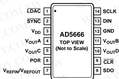
Figure 5. 14-Lead TSSOP (RU-14)
