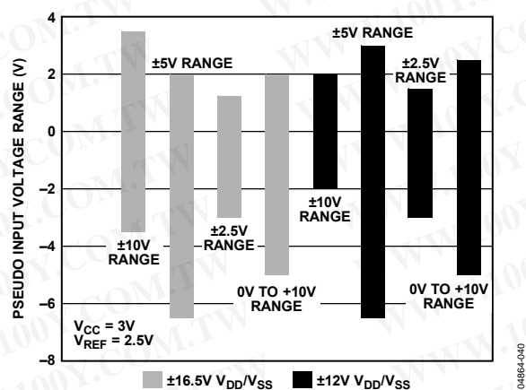
Figure 41. Pseudo Input Range with V_{CC} = 3V
