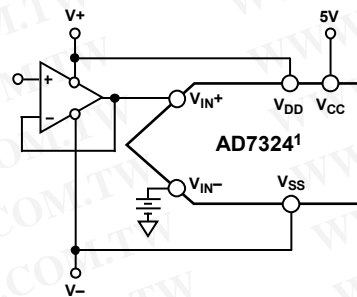
Figure 39. Pseudo Differential Inputs
