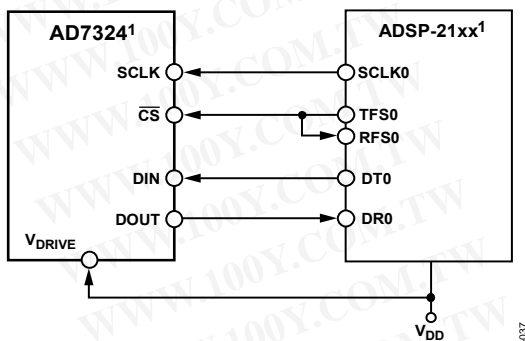
Figure 52. Interfacing the AD7324 to the ADSP-21xx
