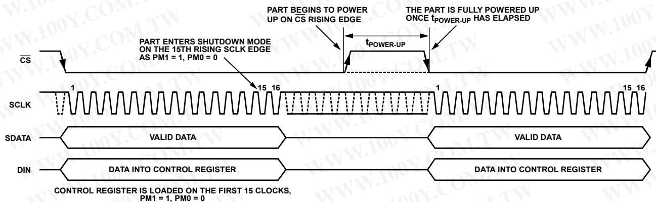
Figure 48. Entering Autos shutdown/Autostandby Mode
