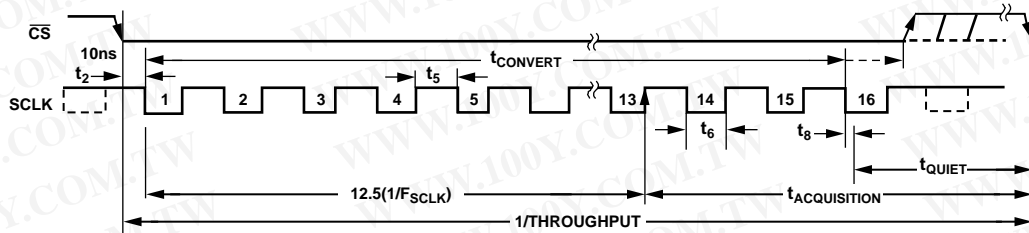
Figure 23. Serial Interface Timing Example
