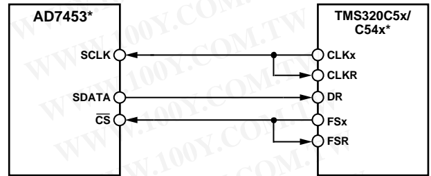
Figure 29. Interfacing to the TMS320C5x/C54x
