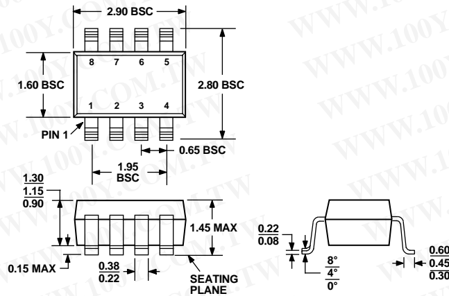
Figure 31. 8-Lead Small Outline Transistor Package [SOT-23] (RT-8) Dimensions shown in millimeters
