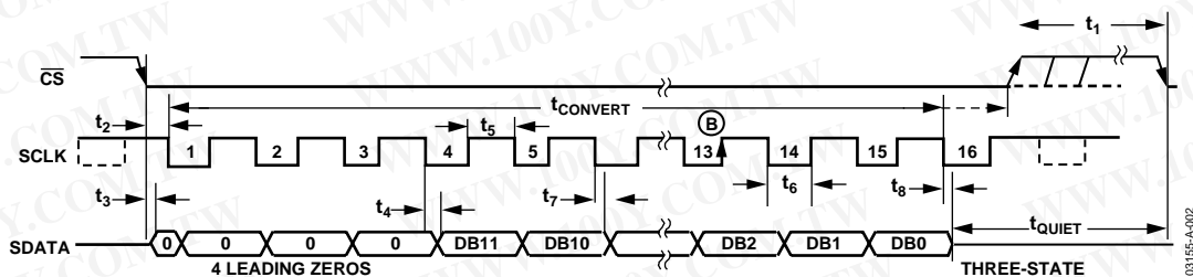
Figure 2. AD7453 Serial Interface Timing Diagram
