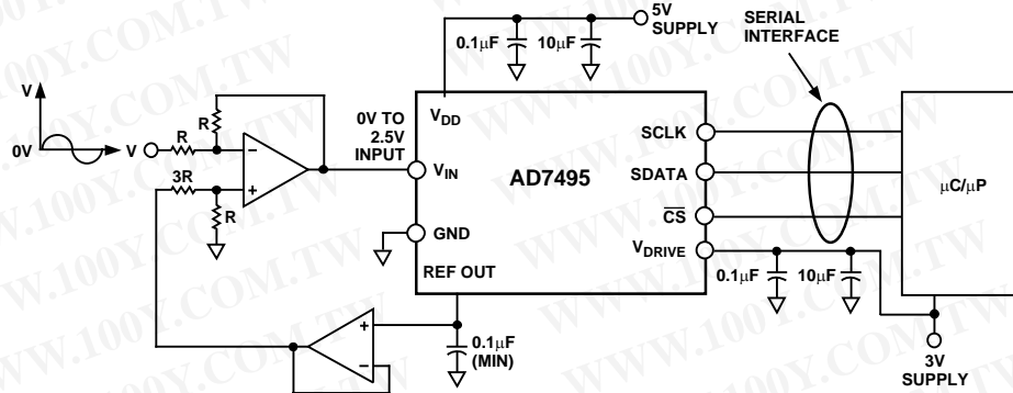
Figure 15. AD7495 Typical Connection Diagram
