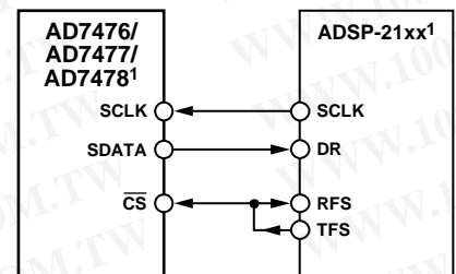
¹ADDITIONAL PINS OMITTED FOR CLARITY Figure 27. Interfacing to the ADSP-21xx
