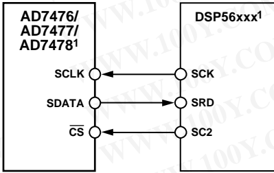
Figure 28. Interfacing to the DSP56xxx
