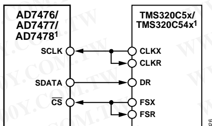
¹ADDITIONAL PINS OMITTED FOR CLARITY Figure 26. Interfacing to the TMS320C5x/C54x
