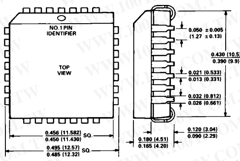
28-Terminal Plastic Leaded Chip Carrier (P-28A)
