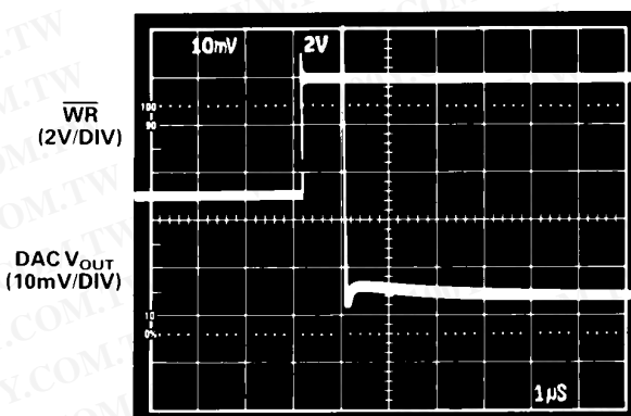
Negative-Going Settling Time ( \pm 2.5 V Range)
