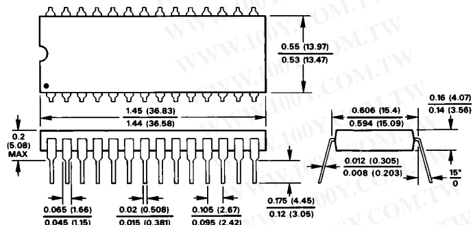
28-Pin Plastic DIP (N-28)
