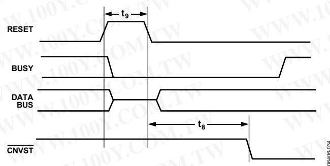
Figure 36. RESET Timing
