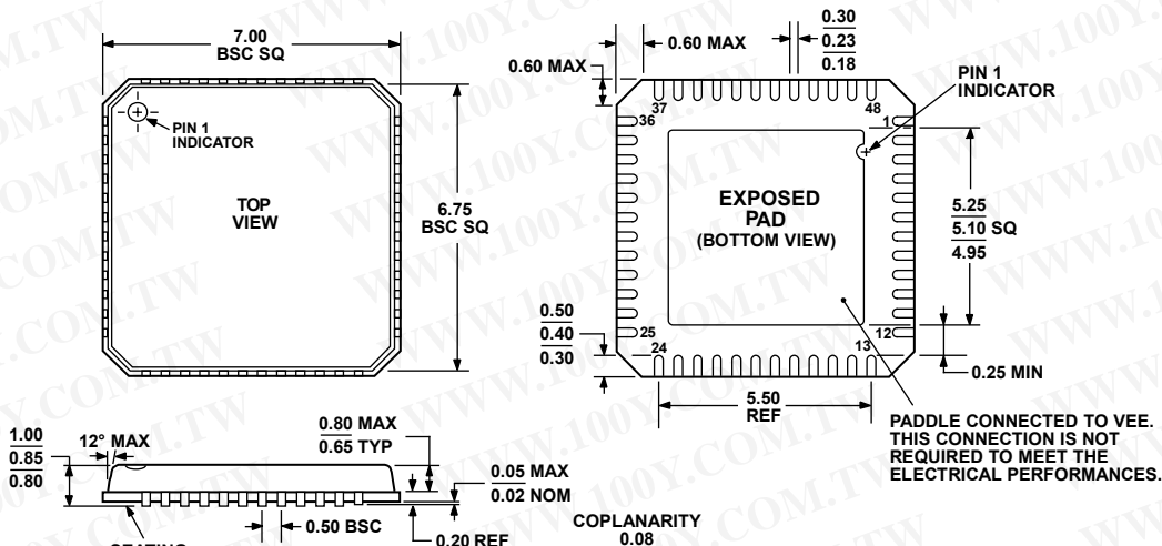
COMPLIANT TO JEDEC STANDARDS MO-220-VKGD-2 Figure 50. 48-Lead Lead Frame Chip Scale Package [LFCSP_VQ] 7 mm x 7 mm Body, Very Thin Quad (CP-48-1) Dimensions shown in millimeters
