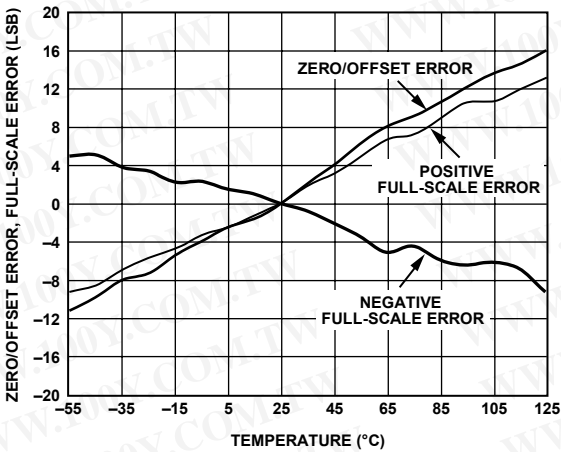
Figure 18. Zero/Offset Error, Positive and Negative Full-Scale Error vs. Temperature, All Normalized to 25°C
