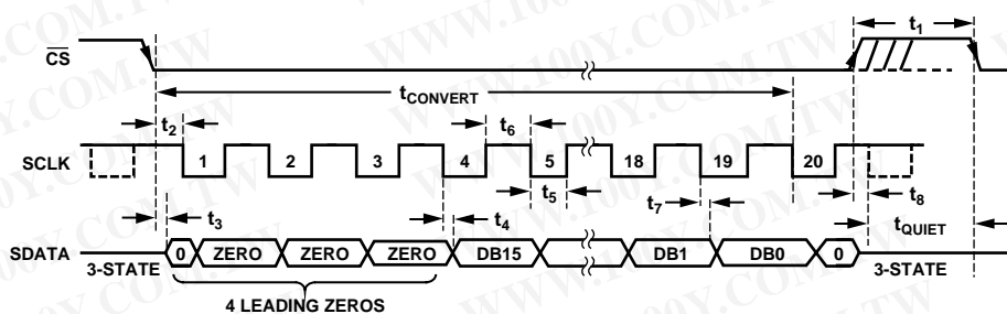
Figure 21. AD7680 Serial Interface Timing Diagram—20 SCLK Transfer
