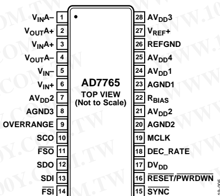
Figure 5. Pin Configuration
