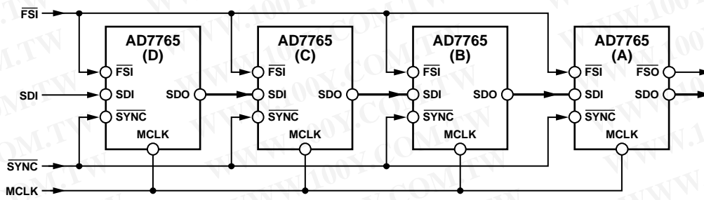
Figure 41. Writing to an AD7765 Daisy-Chain Configuration
