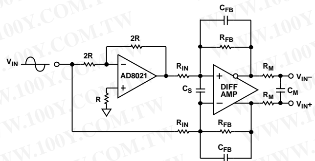
Figure 31. Single-Ended-to-Differential Conversion
