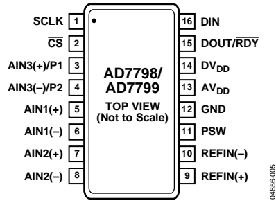
Figure 5. Pin Configuration
