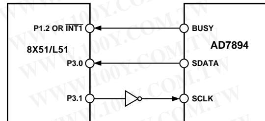
Figure 6. AD7894 to 8X51/L51 Interface
