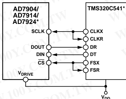
Figure 30. Interfacing to the TMS320C541
