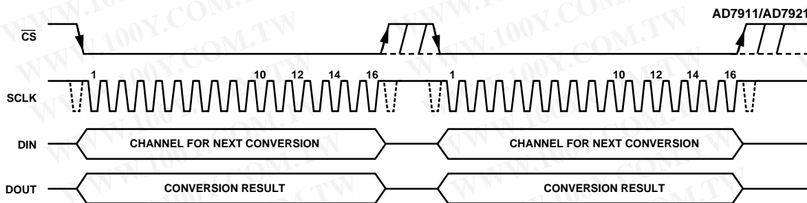
Figure 26. Normal Mode Operation
