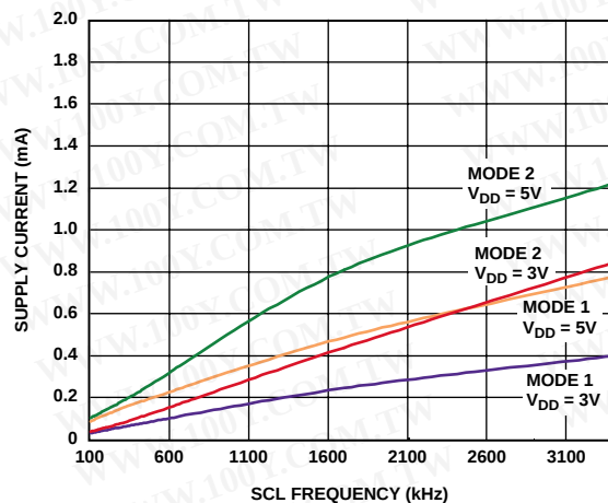
Figure 15. AD7994 Average Supply Current vs. \text{I}^2\text{C} Bus Rate for V_{DD} = 3\text{ V} and 5\text{ V}
