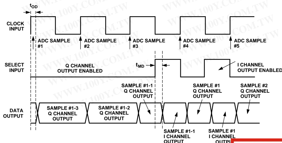
Figure 1. ADC Timing
