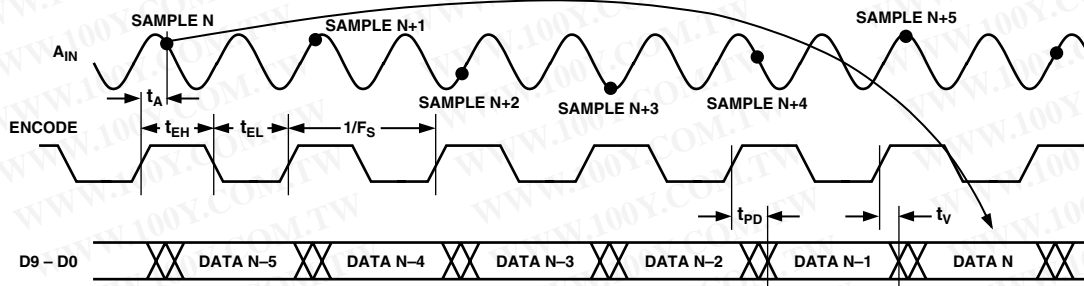
Figure 1. Timing Diagram
