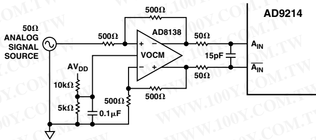
Figure 9. DC-Coupled Analog Input Circuit
