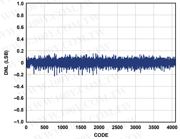
Figure 48. DNL, f_{IN} = 35 MHz, AD9222-65
