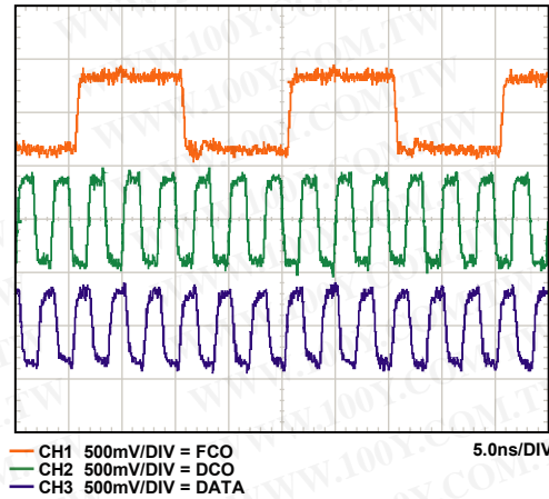
Figure 71. LVDS Output Timing Example in ANSI-644 Mode (Default), AD9222-50
