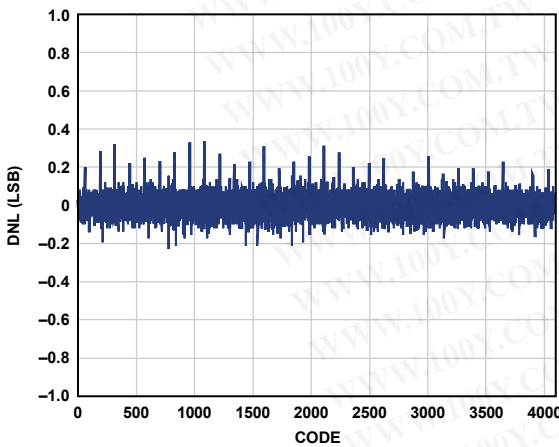
Figure 47. DNL, f_{IN} = 2.3 MHz, AD9222-50
