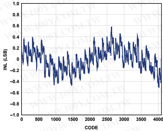
Figure 46. INL, f_{IN} = 35 MHz, AD9222-65
