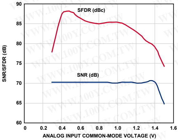
Figure 56. SNR/SFDR vs. Common-Mode Voltage, f_{IN} = 2.3 MHz, AD9222-65
