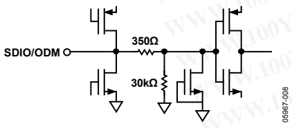
Figure 8. Equivalent SDIO/ODM Input Circuit
