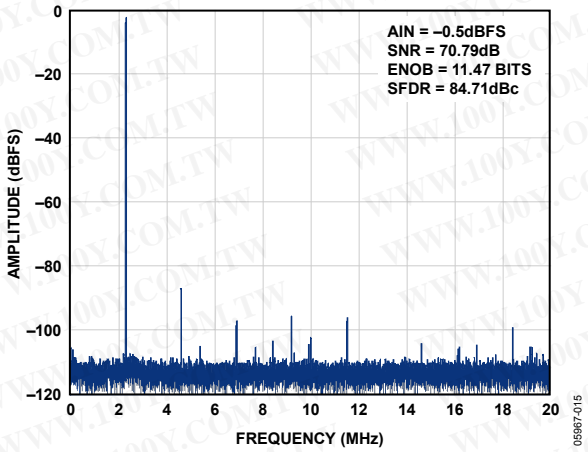
Figure 15. Single-Tone 32k FFT with f_{IN} = 2.3 MHz, AD9222-40
