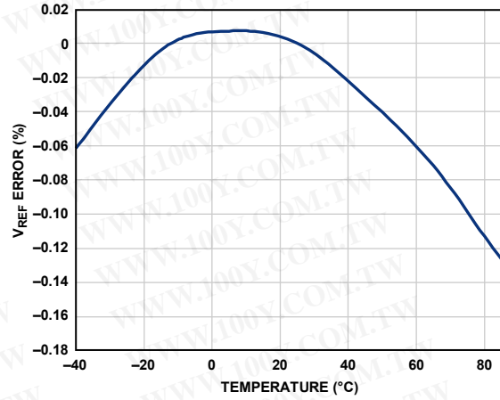
Figure 82. Typical V_{REF} Drift, AD9222-50
