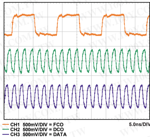
Figure 72. LVDS Output Timing Example in ANSI-644 Mode (Default), AD9222-65
