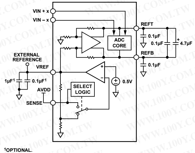
Figure 80. External Reference Operation
