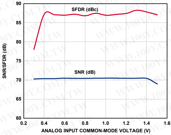
Figure 55. SNR/SFDR vs. Common-Mode Voltage, f_{IN} = 2.3 MHz, AD9222-50
