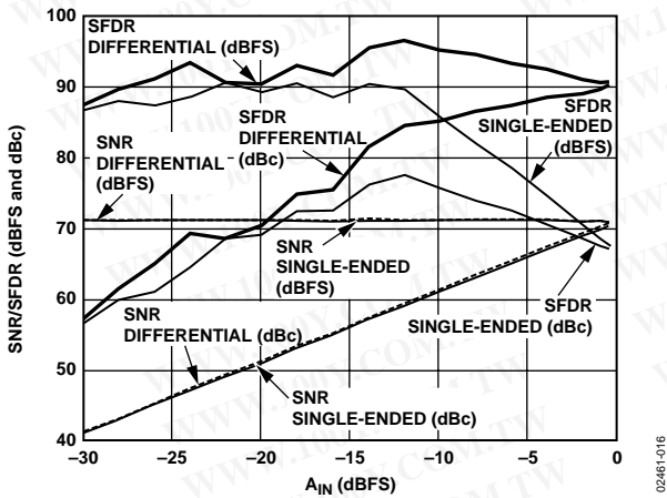
Figure 16. AD9235-40: Single Tone SNR/SFDR vs. A_{IN} with f_{IN} = \text{Nyquist} (20 MHz)
