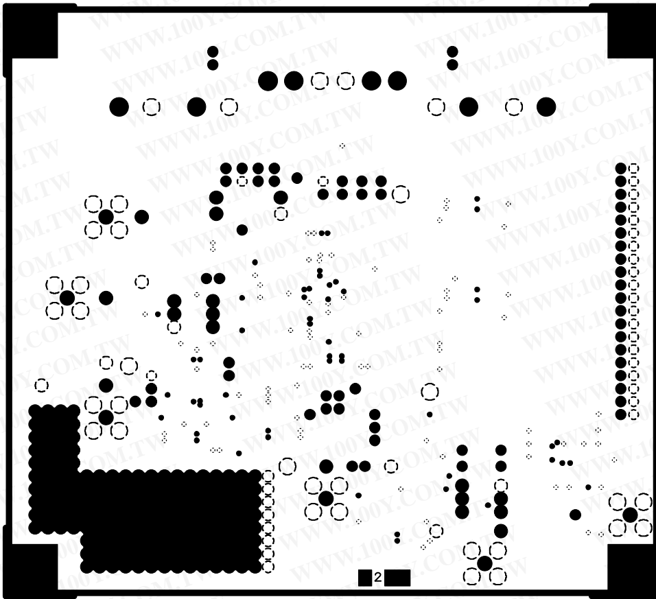
Figure 50. TSSOP Evaluation Board Layout, Ground Plane
