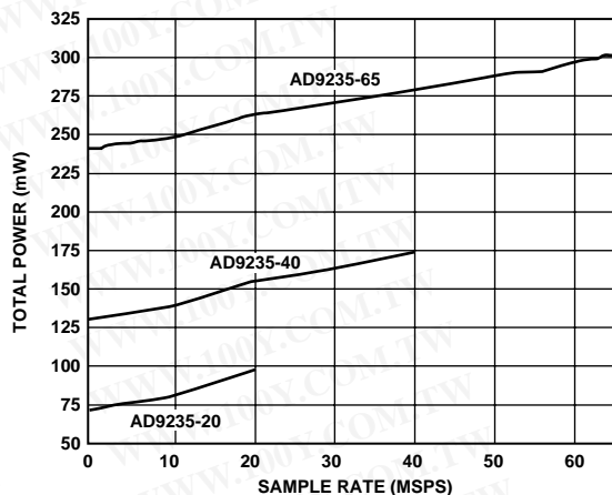
Figure 38. Total Power vs. Sample Rate with f_N = 10 MHz
