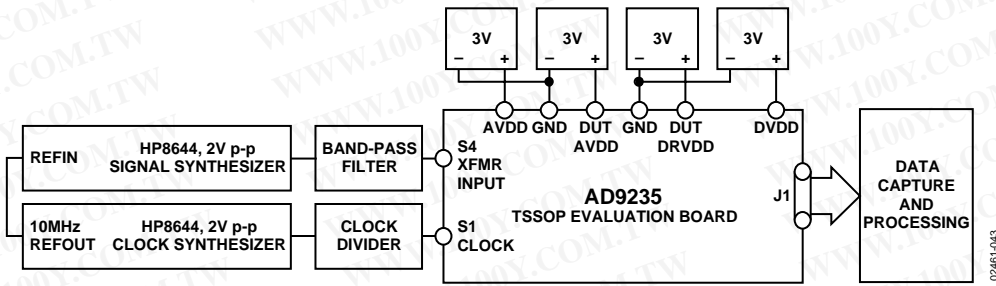
Figure 43. TSSOP Evaluation Board Connections
