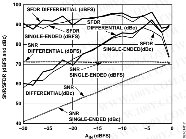
Figure 17. AD9235-20: Single Tone SNR/SFDR vs. A_{IN} with f_{IN} = \text{Nyquist} (10 MHz)
