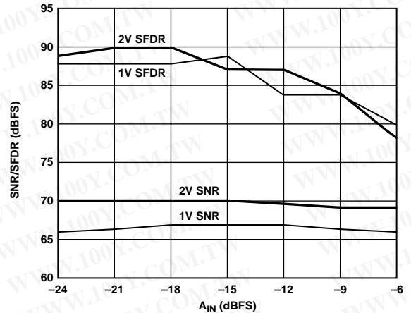
Figure 26. Dual Tone SNR/SFDR vs. A_{IN} with f_{IN1} = 144 MHz and f_{IN2} = 145 MHz
