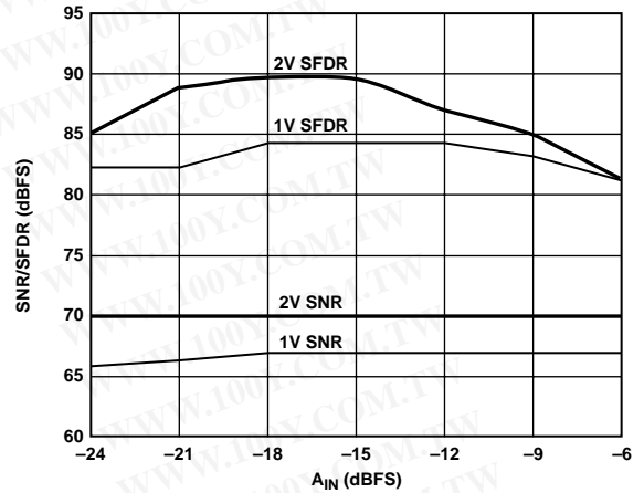
Figure 24. Dual Tone SNR/SFDR vs. A_{IN} with f_{IN1} = 45 MHz and f_{IN2} = 46 MHz
