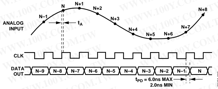
Figure 2. Timing Diagram
