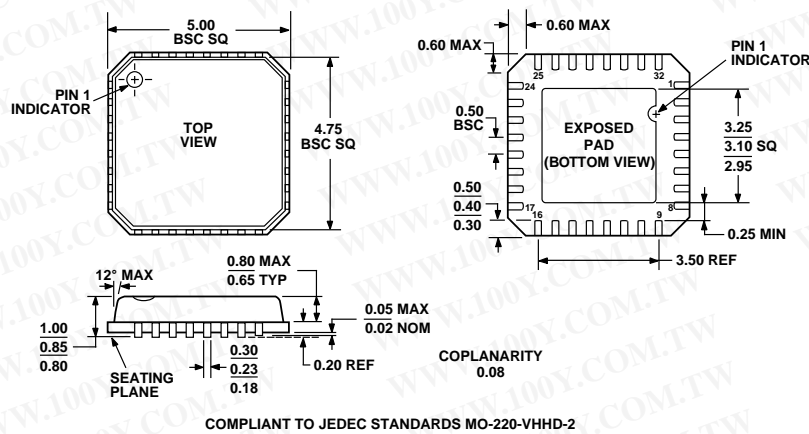
Figure 64. 32-Lead Lead Frame Chip Scale Package [LFCSP] 5 mm x 5 mm Body (CP-32-2) Dimensions shown in millimeters
