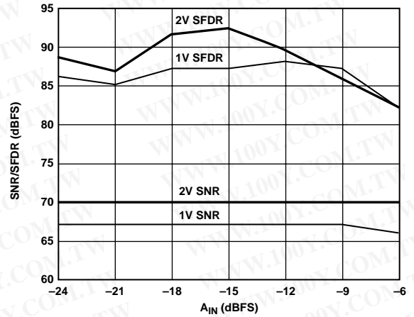
Figure 25. Dual Tone SNR/SFDR vs. A_{IN} with f_{IN1} = 69 MHz and f_{IN2} = 70 MHz
