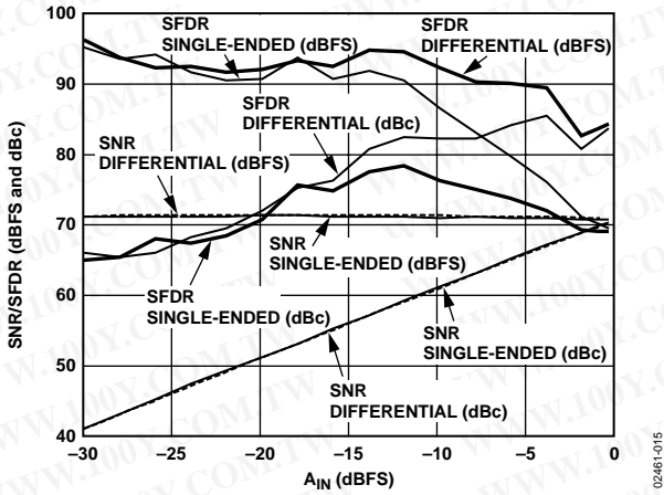
Figure 15. AD9235-65: Single Tone SNR/SFDR vs. A_{IN} with f_{IN} = \text{Nyquist} (32.5 MHz)
