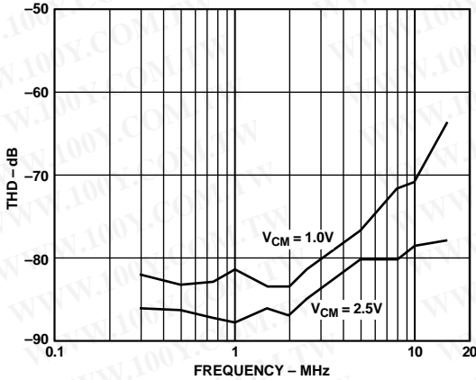
Figure 27. THD vs. Frequency for V_{CM} = 2.5 V and 1.0 V ( A_{IN} = -0.5 dB , Input Span = 2.0 V p-p )
