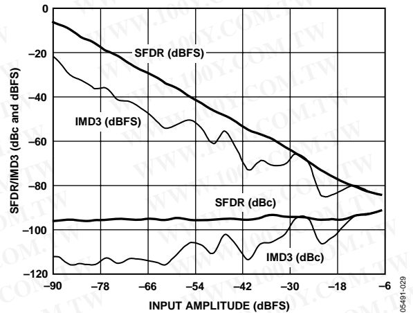
Figure 28. AD9246 Two-Tone SFDR/IMD vs. Input Amplitude ( A_{IN} ) with F_{IN1} = 169.1 MHz, F_{IN2} = 172.11 MHz
