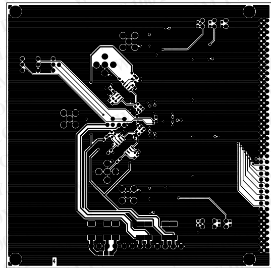
Figure 32. Bottom Routing
