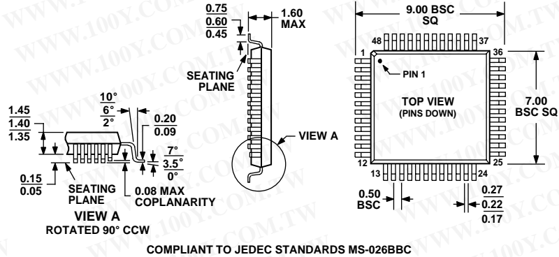
Figure 34. 48-Lead Low Profile Quad Flat Package [LQFP] (ST-48) Dimensions shown in millimeters
