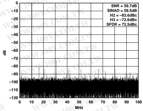
Figure 12. FFT: f_s = 200 MSPS, A_{IN} = 10.3 MHz @ -0.5 dBFS
