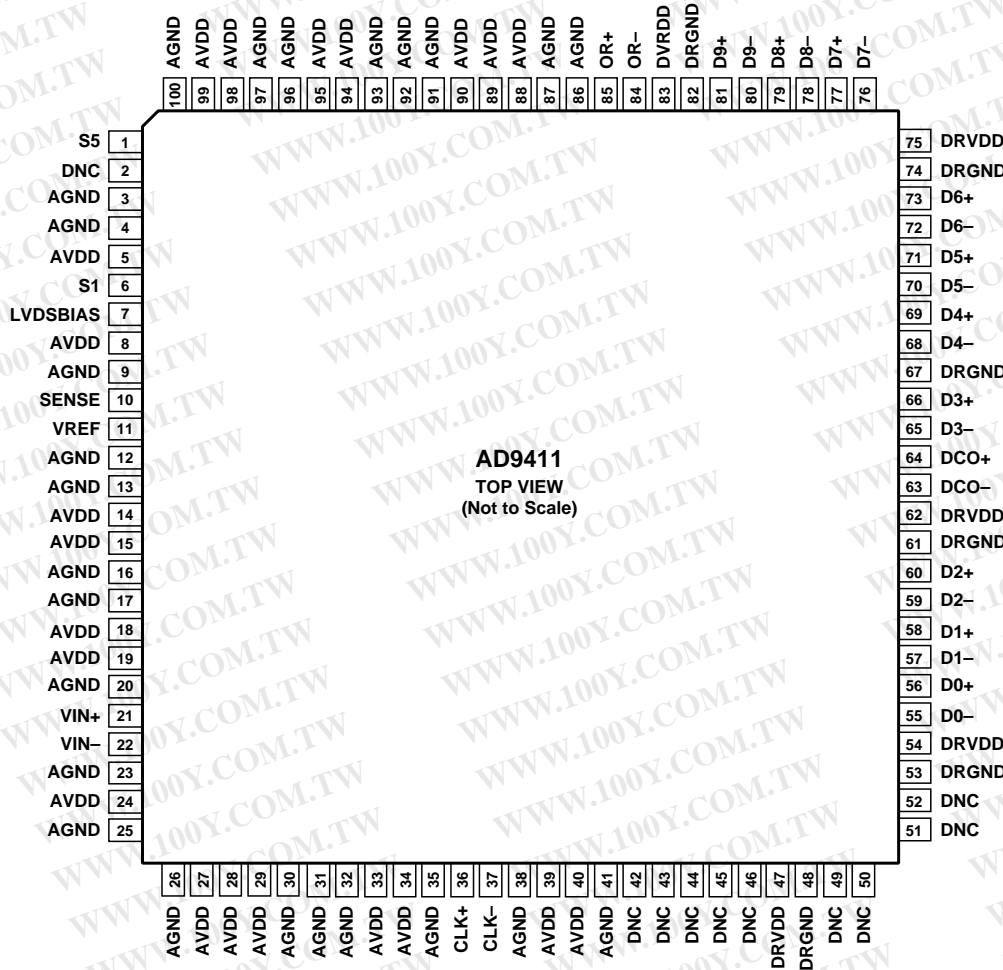
Figure 3. TQFP/EP Pinout
