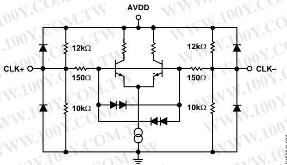
Figure 4. Clock Inputs
