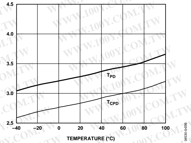
Figure 37. Propagation Delay vs. Temperature (Both Speed Grades)
