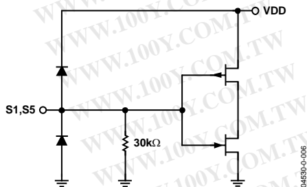
Figure 6. S1 to S5 Inputs
