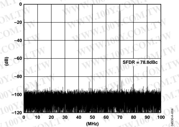
Figure 19. Two-Tone Intermodulation Distortion (69.3 MHz and 70.3 MHz; f_s = 200 MSPS)
