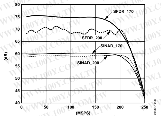
Figure 20. SINAD and SFDR vs. Clock Rate (AIN = 10.3 MHz @ -0.5 dBFS) 170/200 grade
