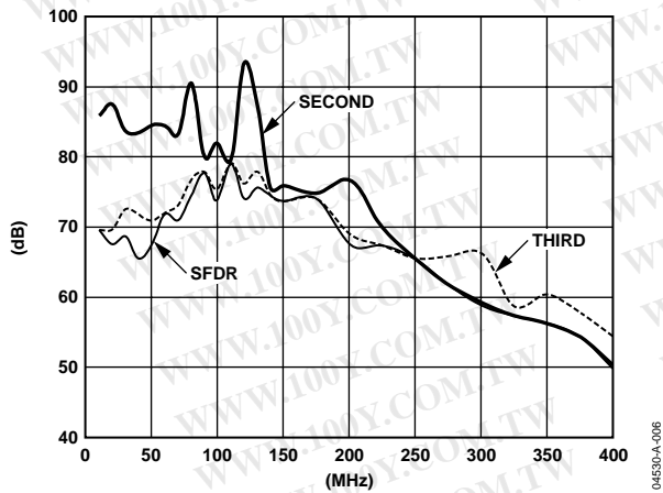
Figure 16. Harmonic Distortion (Second and Third) and SFDR vs. AIN Frequency @ 200 MSPS
