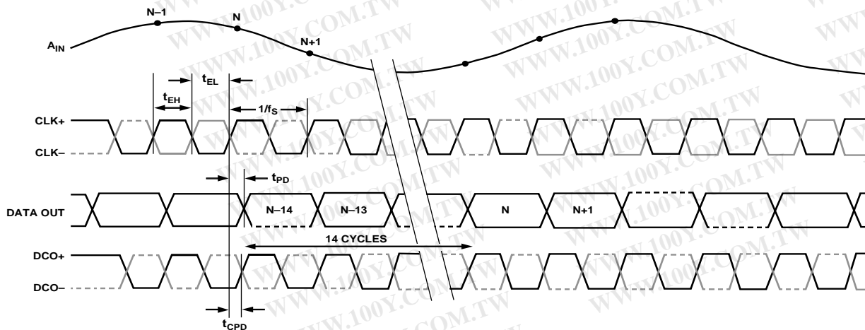
Figure 2. LVDS Timing Diagram
