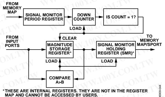
Figure 67. ADC Input Peak Detector Block Diagram
