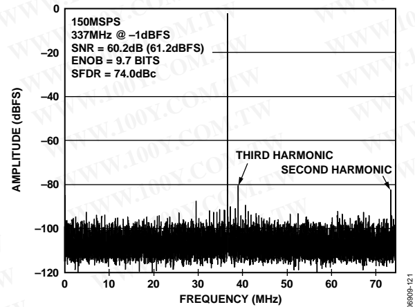
Figure 21. AD9600-150 Single-Tone FFT with f_{IN} = 337 MHz
