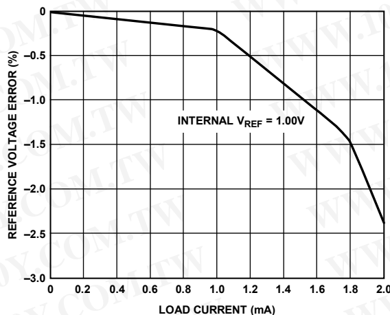
Figure 50. VREF Accuracy vs. Load Current
