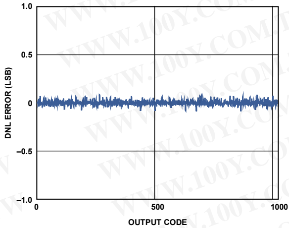
Figure 20. DNL Error with f_{IN} = 9.7 MHz
