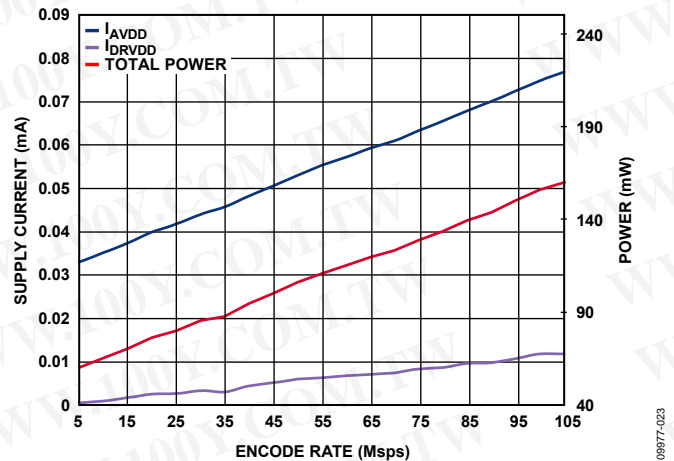
Figure 61. AD9608-105 Power and Current vs. Clock Rate (1.8 V CMOS Output Mode)
