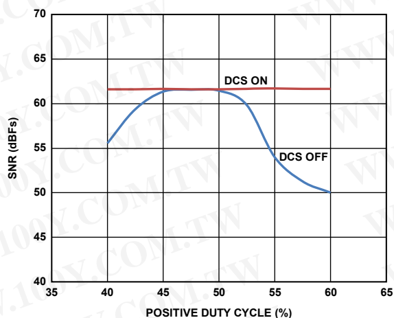
Figure 58. SNR vs. DCS On/Off
