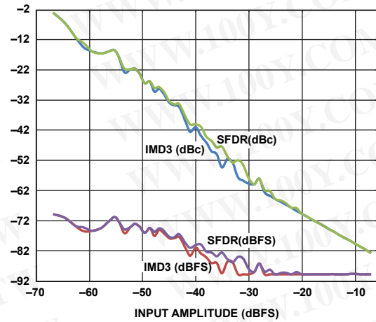
Figure 17. Two-Tone SFDR/IMD3 vs. Input Amplitude (AIN) with f_{IN1} = 29 MHz and f_{IN2} = 32 MHz
