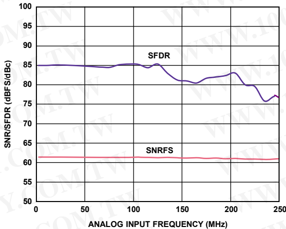
Figure 15. SNR/SFDR vs. Input Frequency (AIN) with 2 V p-p Full Scale
