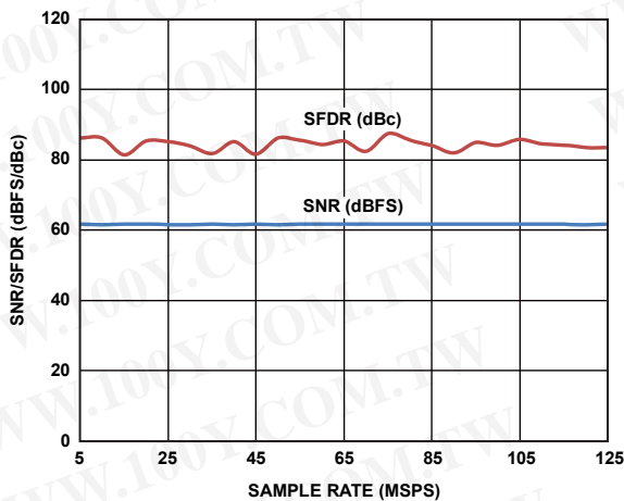
Figure 16. SNR/SFDR vs. Sample Rate with AIN = 9.7 MHz
