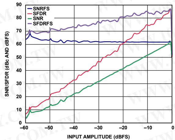
Figure 18. SNR/SFDR vs. Input Amplitude (AIN) with f_{IN} = 9.7 MHz
