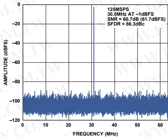
Figure 10. Single-Tone FFT with f_{IN} = 30.5 MHz
