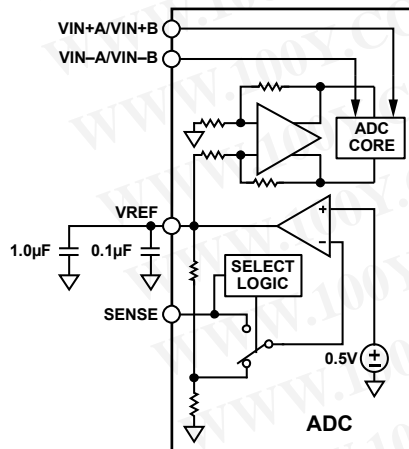
Figure 49. Internal Reference Configuration
