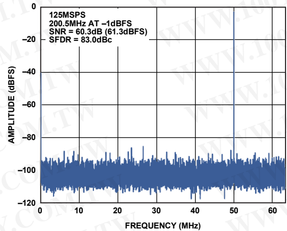
Figure 13. Single-Tone FFT with f_{IN} = 200.5 MHz
