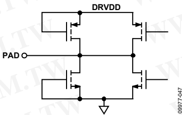
Figure 36. Equivalent Digital Output Circuit
