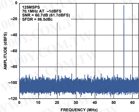
Figure 11. Single-Tone FFT with f_{IN} = 70.1 MHz
