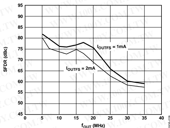
Figure 31. SFDR vs. f_{OUT} and I_{OUTFS} @ 80 MSPS
