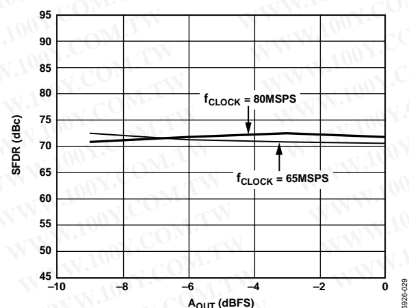
Figure 32. SFDR vs. A_{OUT} @ f_{OUT} = f_{CLOCK}/5
