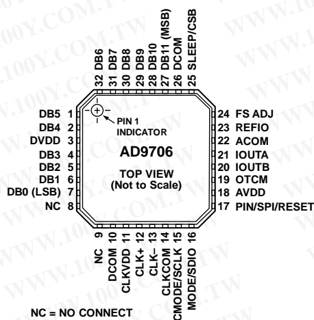
Figure 4. AD9706 Pin Configuration
