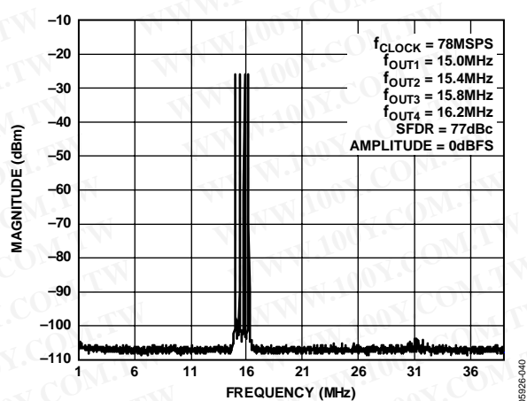
Figure 43. Four-Tone SFDR
