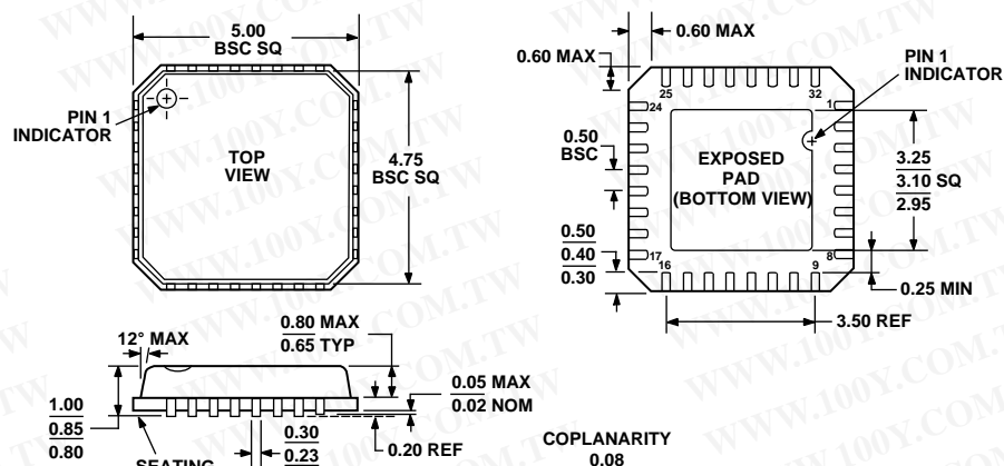
Figure 103. 32-Lead Lead Frame Chip Scale Package [LFCSP_VQ]
