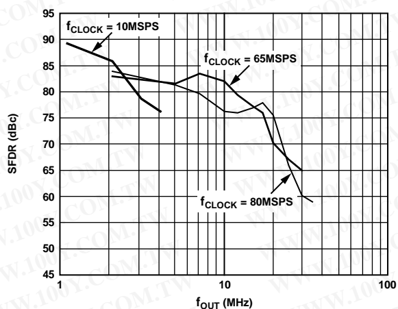
Figure 27. SFDR vs. f_{OUT}
