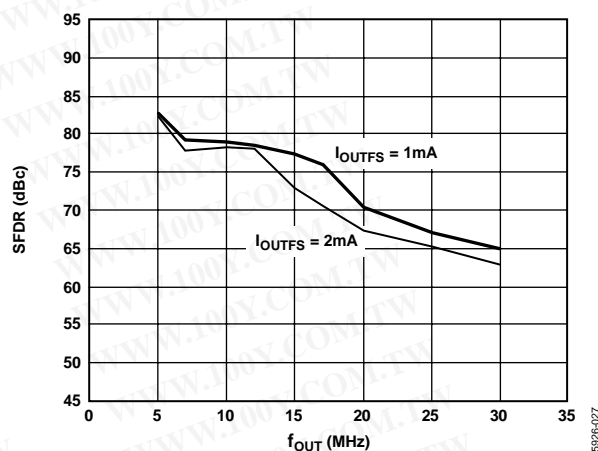
Figure 30. SFDR vs. f_{OUT} and I_{OUTFS} @ 65 MSPS
