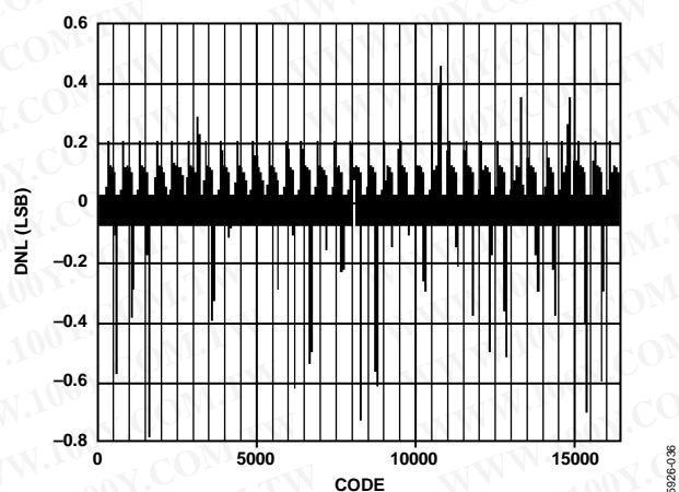
Figure 39. Typical Uncalibrated DNL
