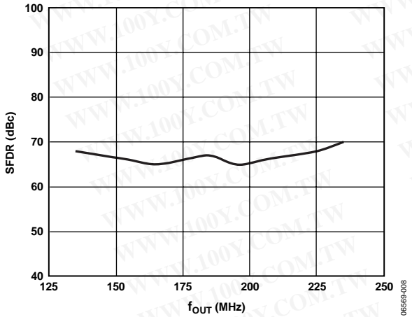
Figure 8. AD9747 SFDR vs. f_{OUT} , Mix Mode, 250 MSPS
