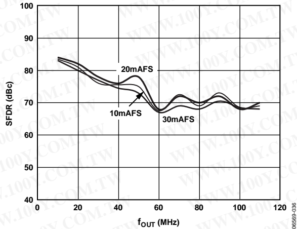
Figure 13. AD9747 SFDR vs. Analog Output, 250 MSPS
