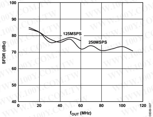
Figure 7. AD9747 SFDR vs. f_{OUT} , Normal Mode
