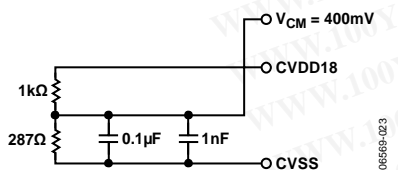
Figure 32. DAC Clock VCM Circuit
