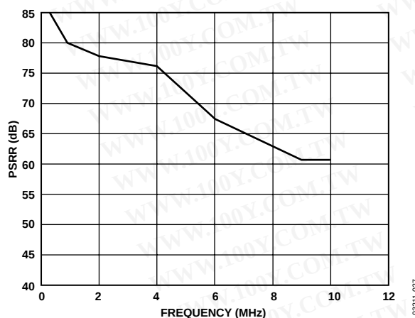
Figure 30. Power Supply Rejection Ratio (PSRR)
