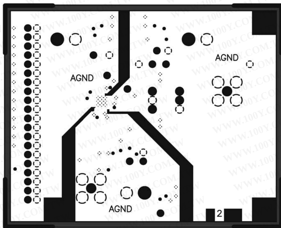
Figure 37. Evaluation Board Layout—Ground Plane
