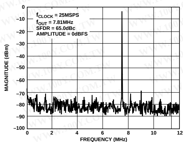
Figure 10. Single-Tone Spectral Plot @ 25 MSPS (Single-Ended Output)
