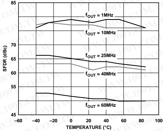
Figure 18. SFDR vs. Temperature @ f_{CLK} = 125 MSPS, 0 dBFS
