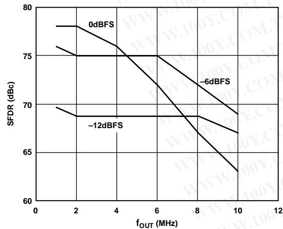
Figure 8. SFDR vs. f OUT @ 25 MSPS
