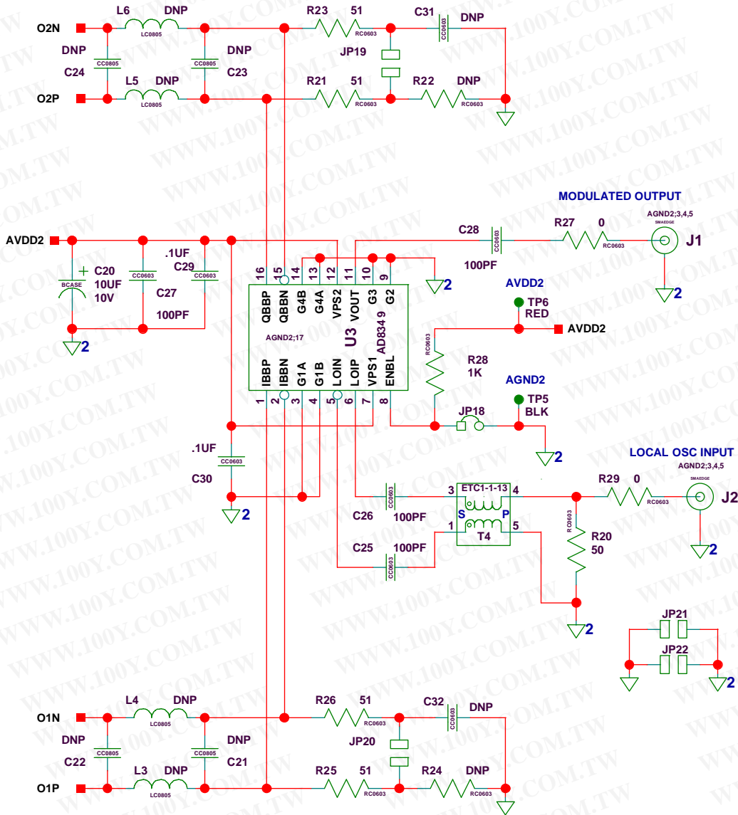
Figure 88. Modulator on AD9763/AD9765/AD9767 Evaluation Board
