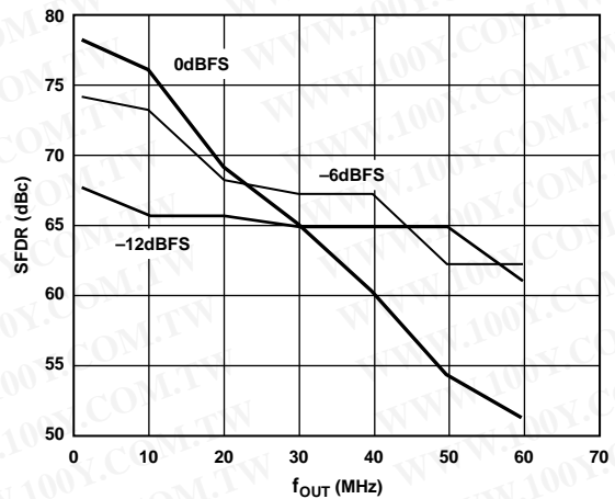
Figure 10. SFDR vs. f OUT @ 125 MSPS
