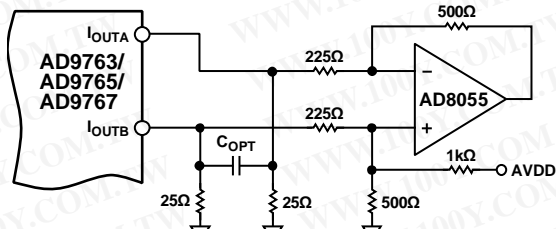
Figure 74. Single-Supply DC Differential-Coupled Circuit
