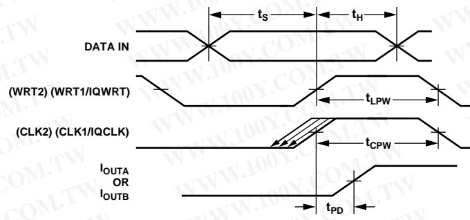
Figure 2. Timing Diagram for Dual and Interleaved Modes
