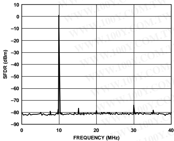
Figure 20. Single-Tone SFDR @ f_{CLK} = 125 MSPS
