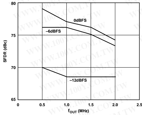
Figure 7. SFDR vs. f OUT @ 5 MSPS
