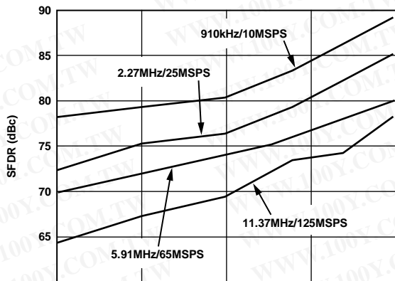
Figure 46. Single-Tone SFDR vs. A_{OUT} @ f_{OUT} = f_{CLK}/11
