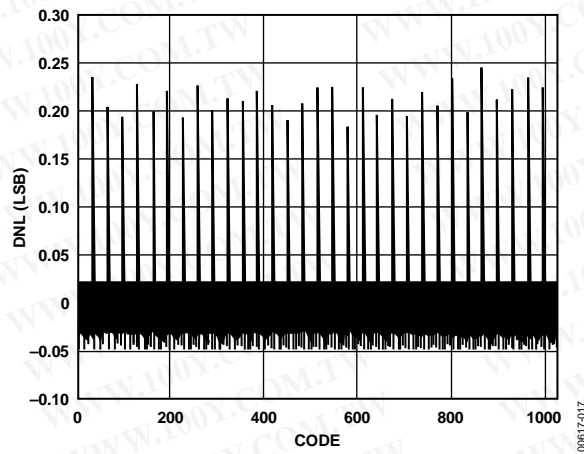
Figure 17. Typical DNL
