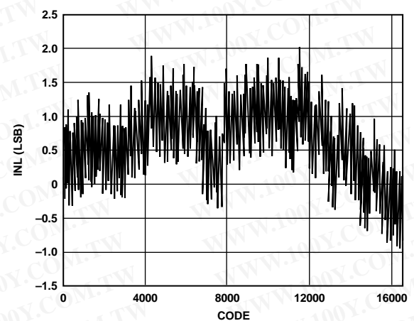
Figure 50. Typical INL
