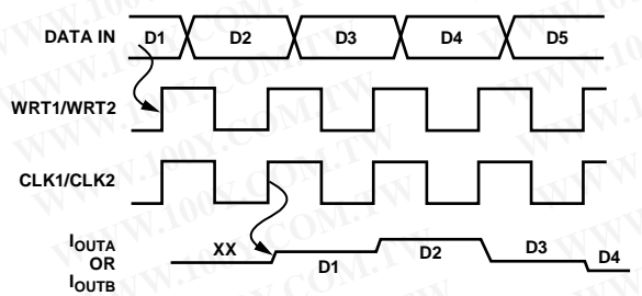
Figure 63. Dual-Port Mode Timing
