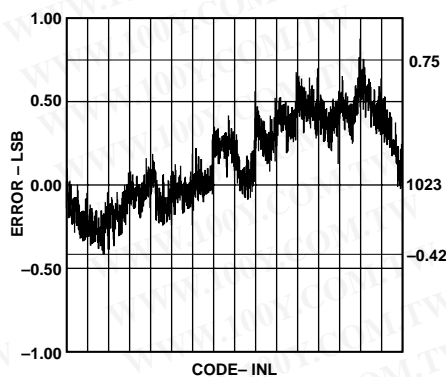
Figure 16. Typical Linearity
