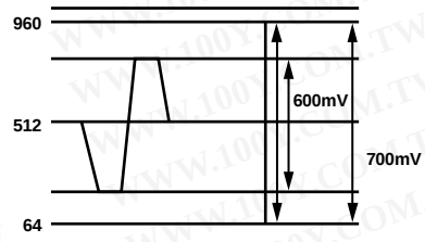
Figure 129. EIA-770.3 Standard Output Signals (1080i/720p)
