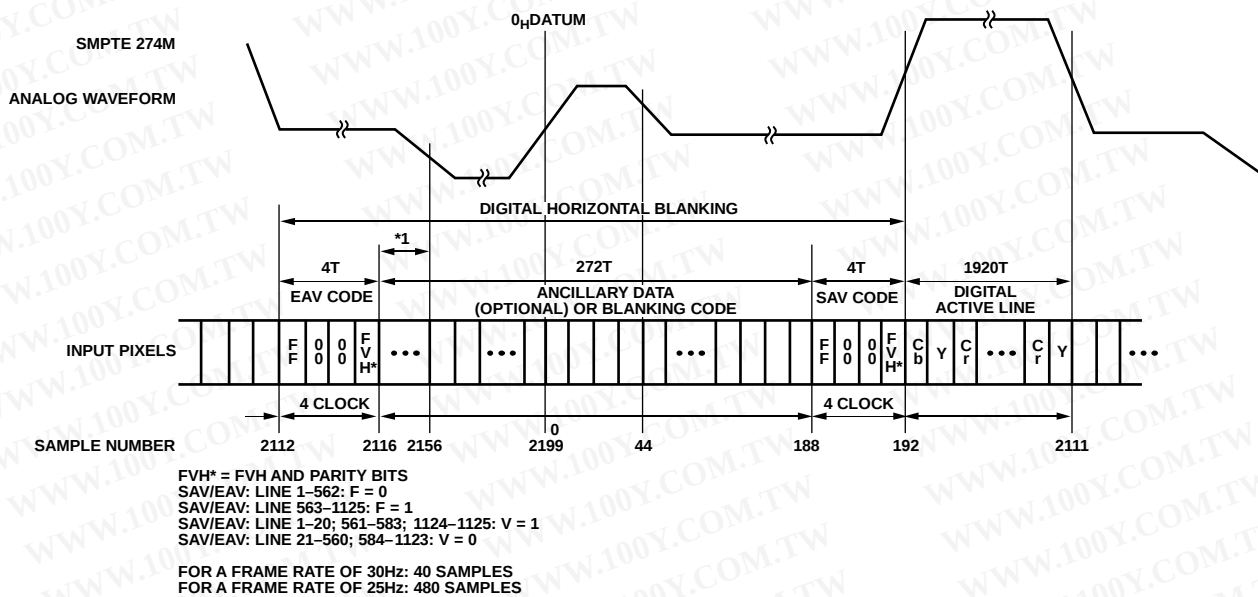
Figure 141. EAV/SAV Input Data Timing Diagram (SMPTE 274M)
