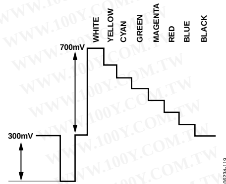
Figure 124. Y Levels—PAL
