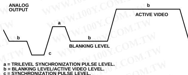
Figure 63. ED/HD Nonstandard Timing Mode Output Levels
