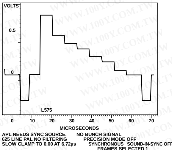
Figure 139. PAL Luma
