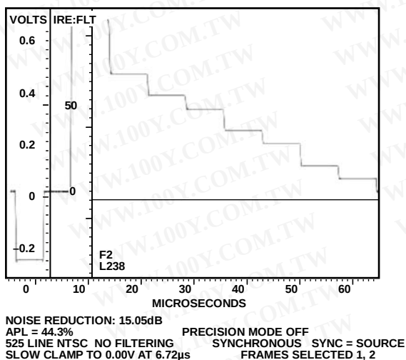
Figure 136. NTSC Luma
