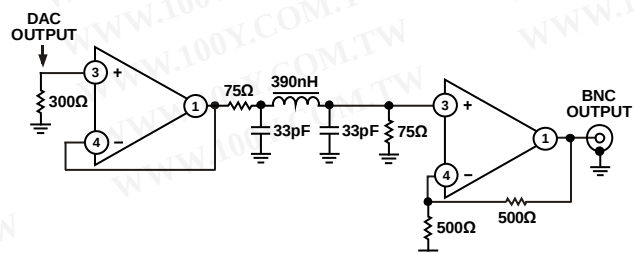
Figure 92. Example of Output Filter for HD, 4 \times Oversampling
