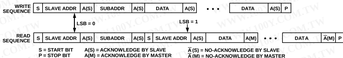
Figure 50. I²C Read and Write Sequence
