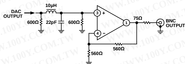
Figure 90. Example of Output Filter for SD, 16 \times Oversampling
