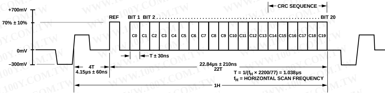
Figure 102. High Definition (1080i) CGMS Waveform
