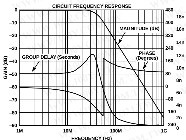
Figure 94. Output Filter Plot for ED, 8x Oversampling
