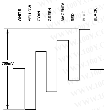
Figure 123. Pb Levels—NTSC
