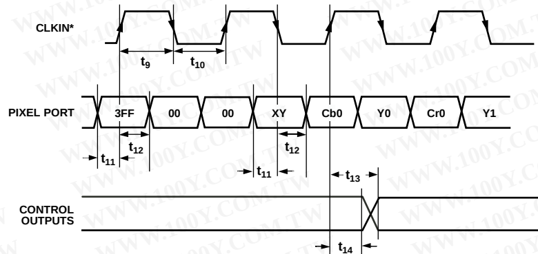
Figure 9. ED/HD-DDR Input, 8-/10-Bit 4:2:2 YCrCb (EAV/SAV), Input Mode 010
