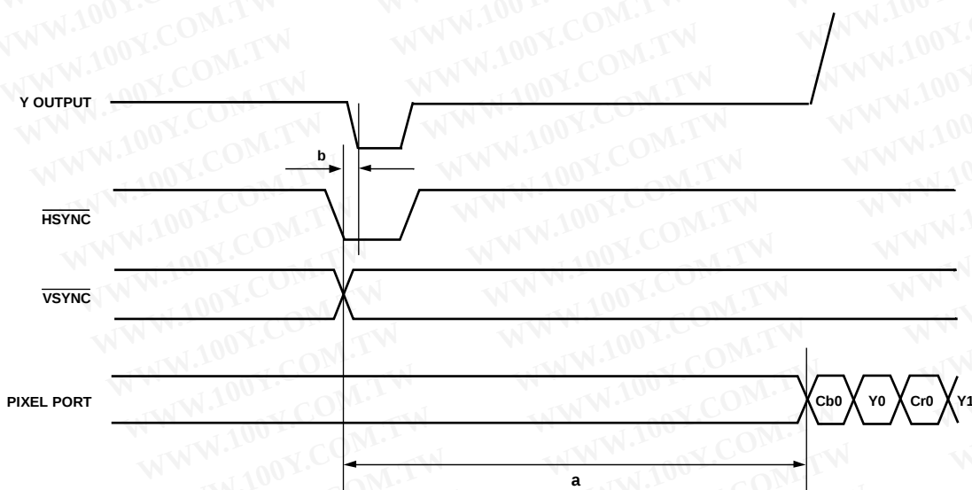
Figure 12. ED-SDR, 16-Bit 4:2:2 YCrCb (HSYNC/VSYNC) Input Timing Diagram
