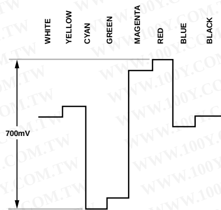
Figure 125. Pr Levels—PAL
