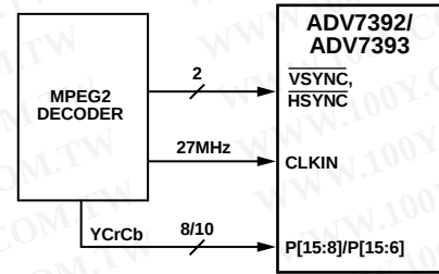
Figure 56. SD Example Application
