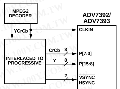
Figure 59. ED/HD-SDR Example Application
