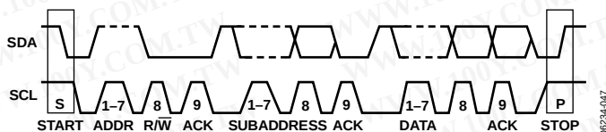
Figure 49. I²C Data Transfer
