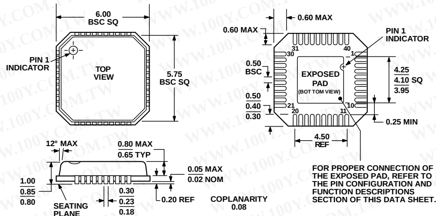
COMPLIANT TO JEDEC STANDARDS MO-220-VJJD-2 Figure 149. 40-Lead Lead Frame Chip Scale Package [LFCSP_VQ] 6 mm x 6 mm Body, Very Thin Quad (CP-40-1) Dimensions shown in millimeters
