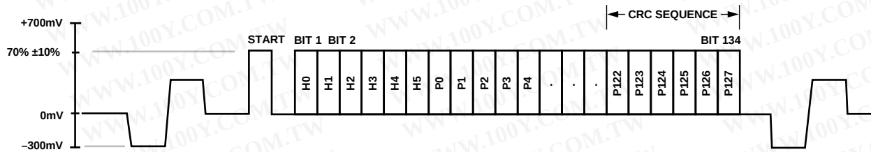
Figure 103. Enhanced Definition (525p) CGMS Type B Waveform
