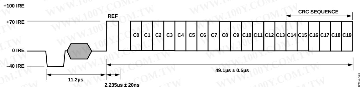
Figure 98. Standard Definition CGMS Waveform
