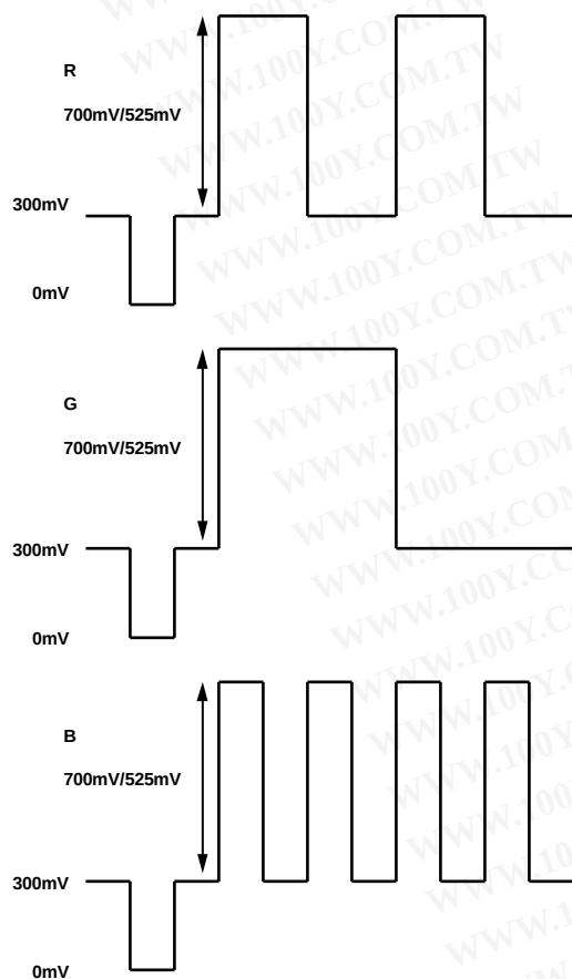
Figure 132. SD/ED RGB Output Levels—RGB Sync Enabled
