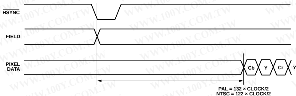
Figure 113. SD Timing Mode 1, Odd/Even Field Transitions (Master/Slave)
