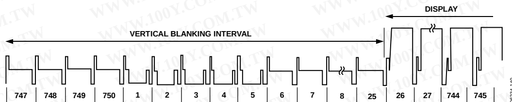
Figure 145. SMPTE 296M (720p)
