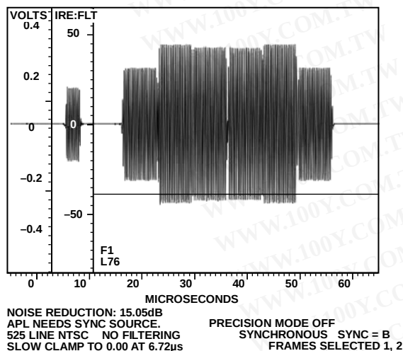
Figure 137. NTSC Chroma
