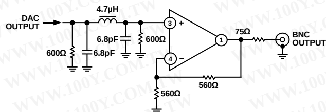
Figure 91. Example of Output Filter for ED, 8 \times Oversampling
