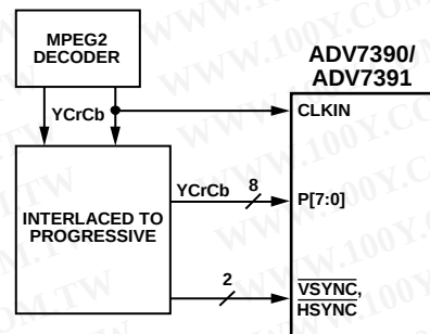
Figure 54. ED/HD-DDR Example Application
