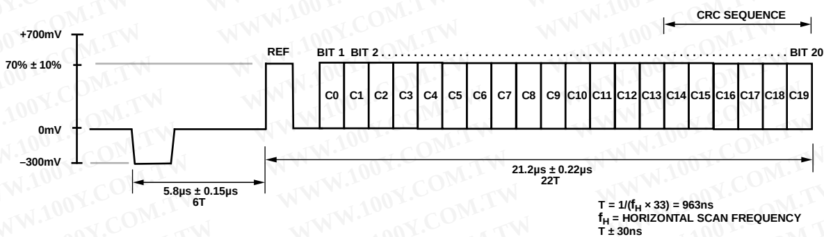
Figure 99. Enhanced Definition (525p) CGMS Waveform
