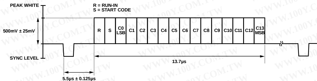
Figure 100. Enhanced Definition (625p) CGMS Waveform
