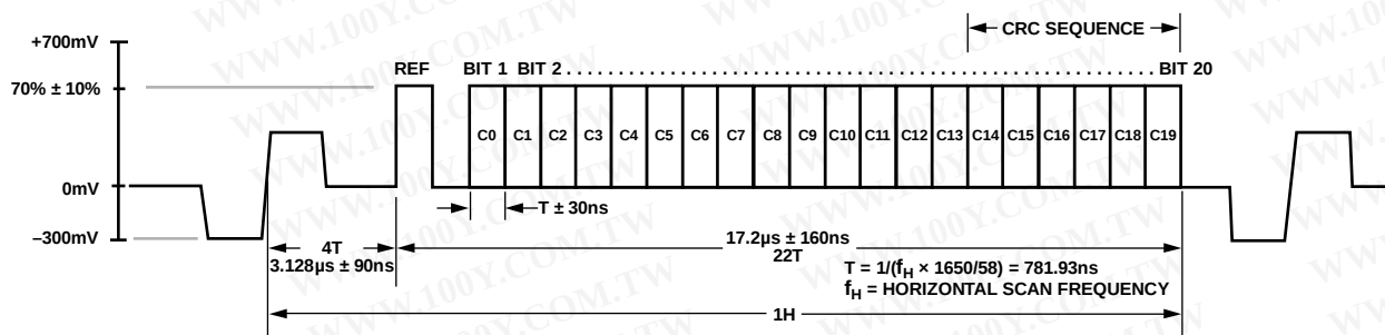
Figure 101. High Definition (720p) CGMS Waveform
