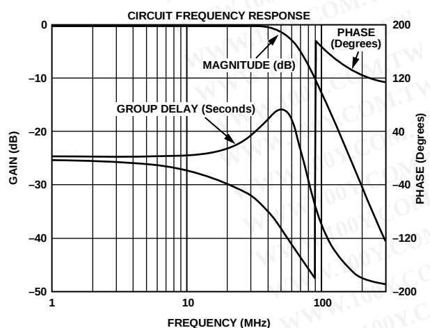
Figure 95. Output Filter Plot for HD, 4x Oversampling
