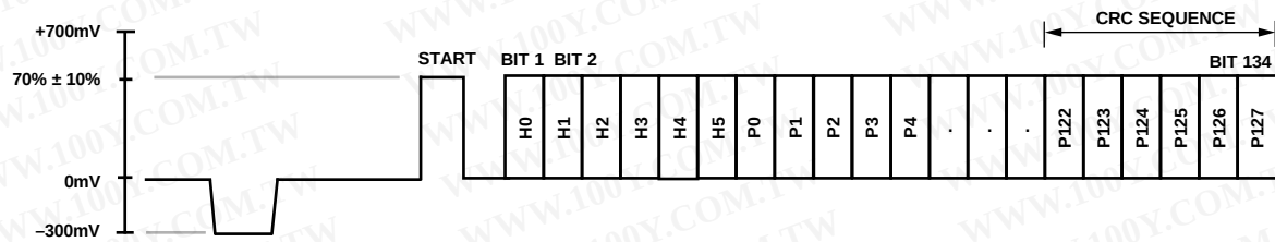
Figure 103. Enhanced Definition (525p) CGMS Type B Waveform
