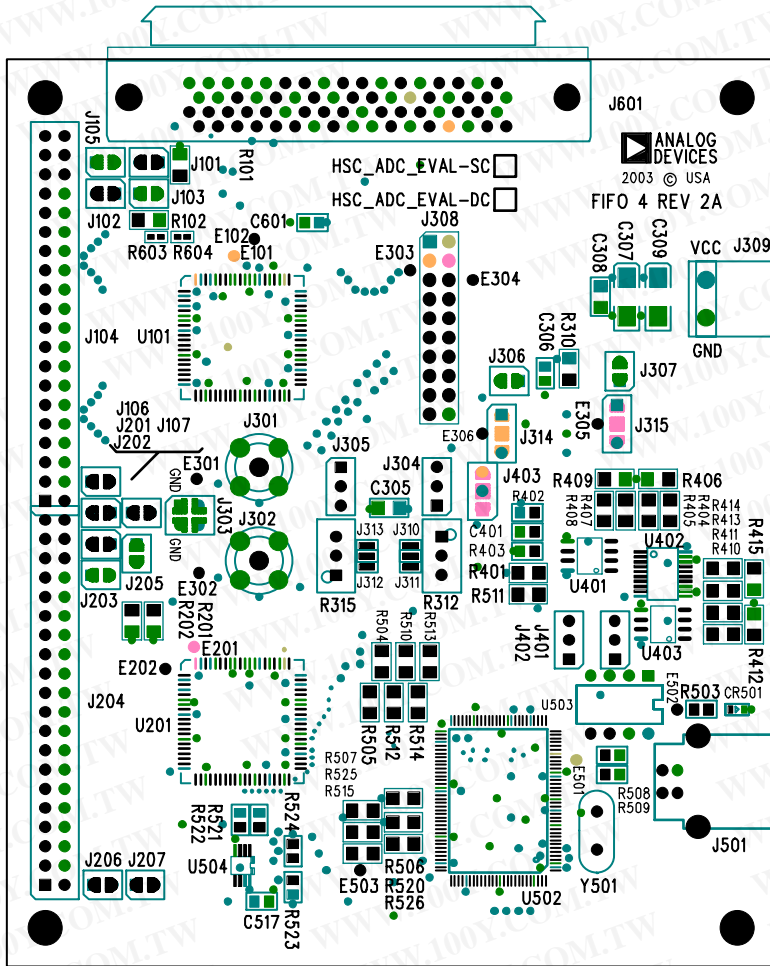
Figure 34. Assembly—Primary Side
