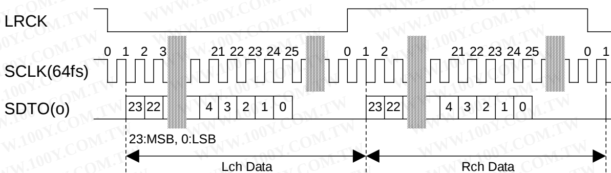
Figure 2. Mode 1 Timing
