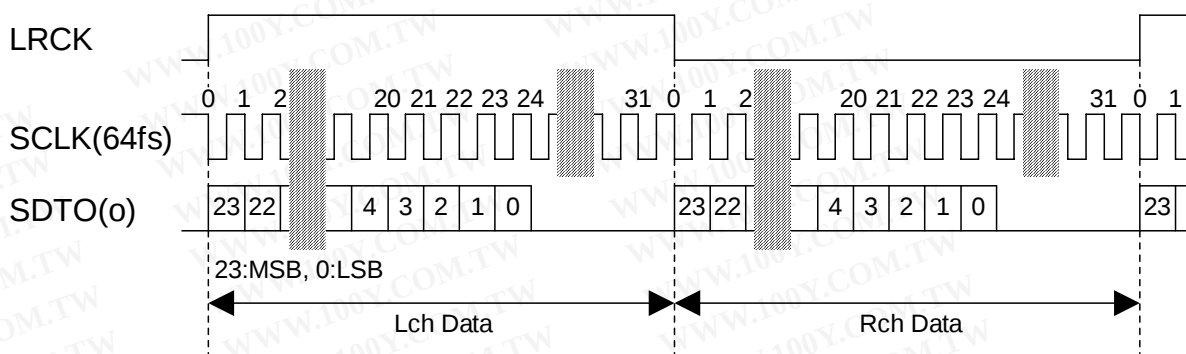
Figure 1. Mode 0 Timing
