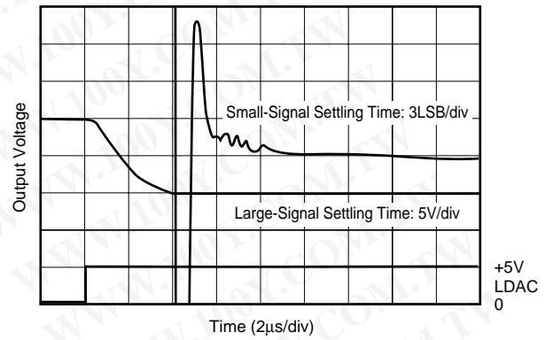
OUTPUT VOLTAGE vs SETTTLING TIME (+10V to 0V)
