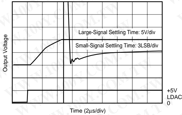
OUTPUT VOLTAGE vs SETTTLING TIME (0V to +10V)
