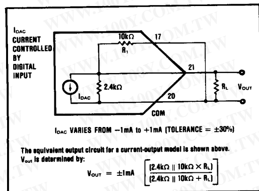
FIGURE 12. Driving a Resistive Load With PCM53-1.
