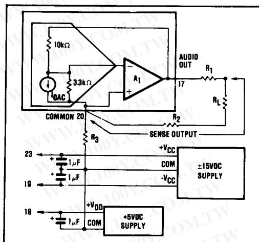
FIGURE 10. Output Circuit for PCM53-V.
