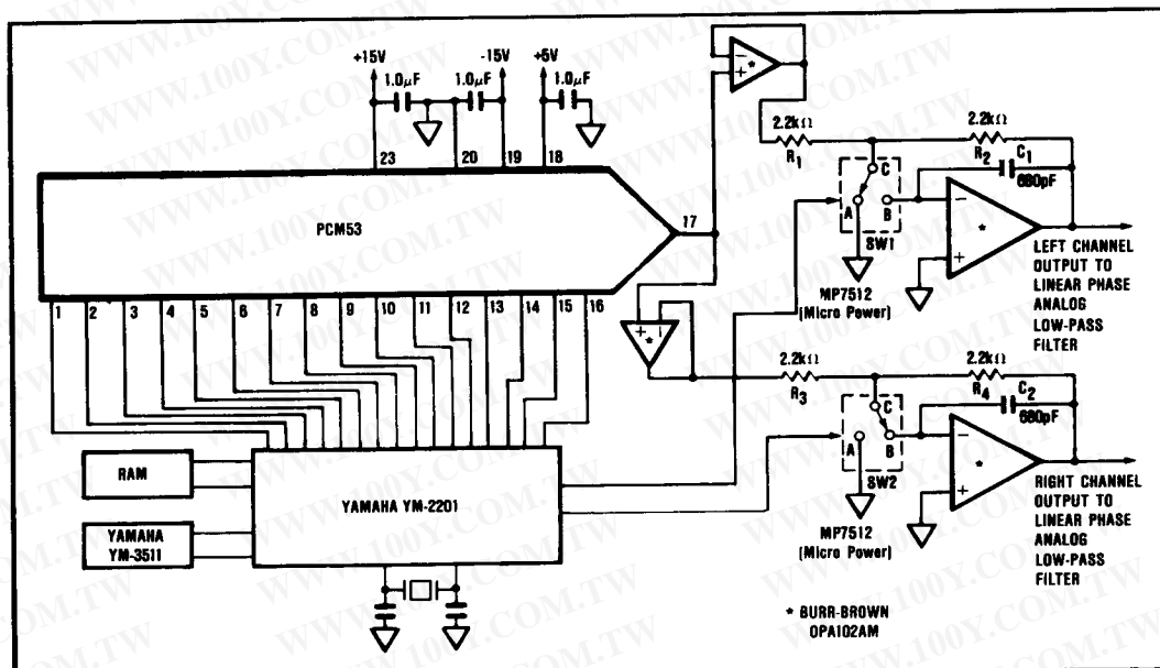
FIGURE 17. Oversampling Digital-Filter Technique Using Yamaha LSI.
