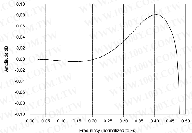
Figure 18. Passband Ripple
