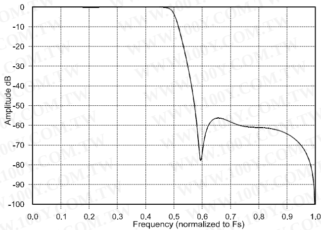
Figure 19. Stopband Rejection
