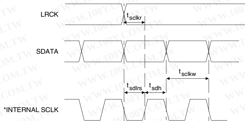
Figure 5. Internal Serial Mode Input Timing
