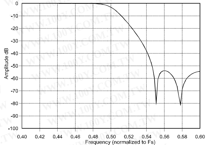
Figure 16. Transition Band
