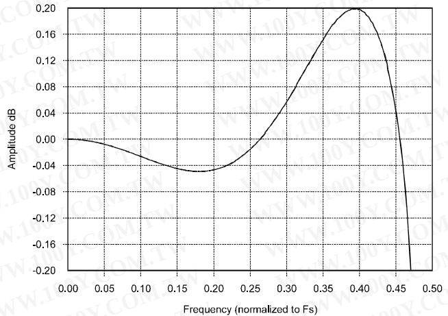
Figure 22. Passband Ripple
