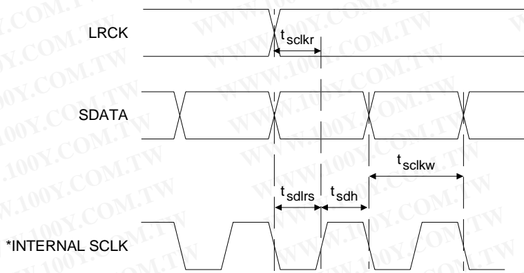
Figure 3. External Serial Mode Input Timing
