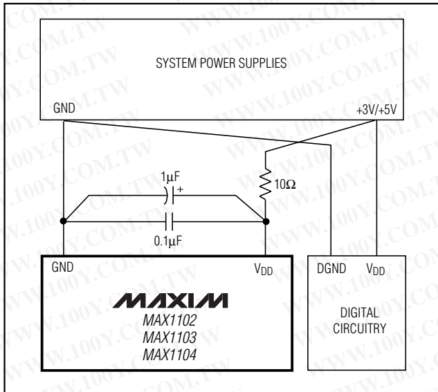
Figure 10. Power-Supply Connections
