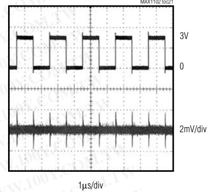
CLOCK FEEDTHROUGH
