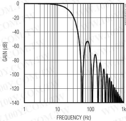
NORMAL-MODE FREQUENCY RESPONSE (MAX11212B)
