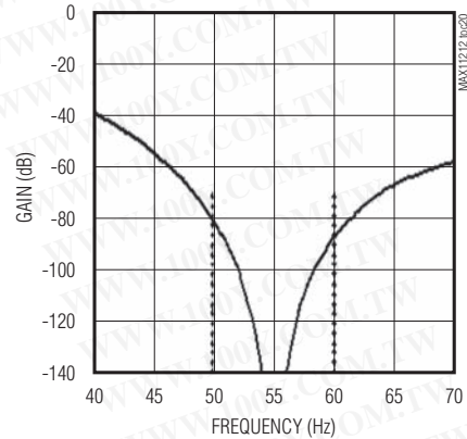
NORMAL-MODE REJECTION OF 50Hz TO 60Hz (MAX11212B)
