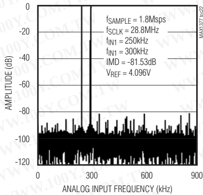
MAX1379 INTERMODULATION PLOT
