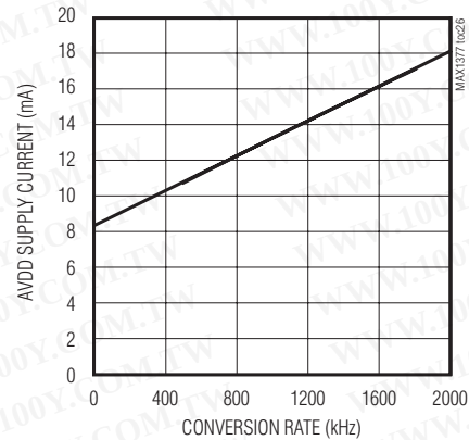
MAX1379 AVDD SUPPLY CURRENT vs. CONVERSION RATE
