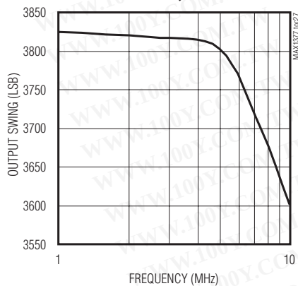
MAX1379 FULL-SCALE AMPLITUDE vs. FREQUENCY
