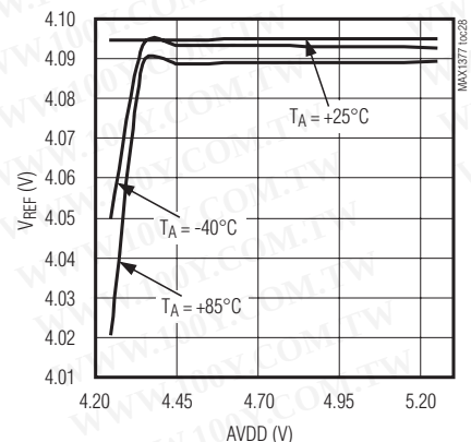
MAX1379 INTERNAL REFERENCE VOLTAGE vs. ANALOG SUPPLY VOLTAGE
