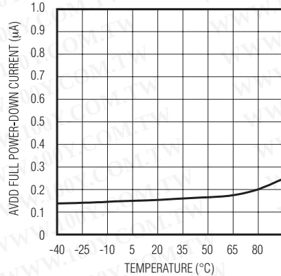
MAX1379 AVDD FULL POWER-DOWN CURRENT vs. TEMPERATURE
