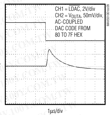
WORST-CASE 1LSB DIGITAL STEP CHANGE (NEGATIVE)
