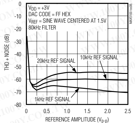
TOTAL HARMONIC DISTORTION PLUS NOISE AT DAC OUTPUT vs. REFERENCE AMPLITUDE
