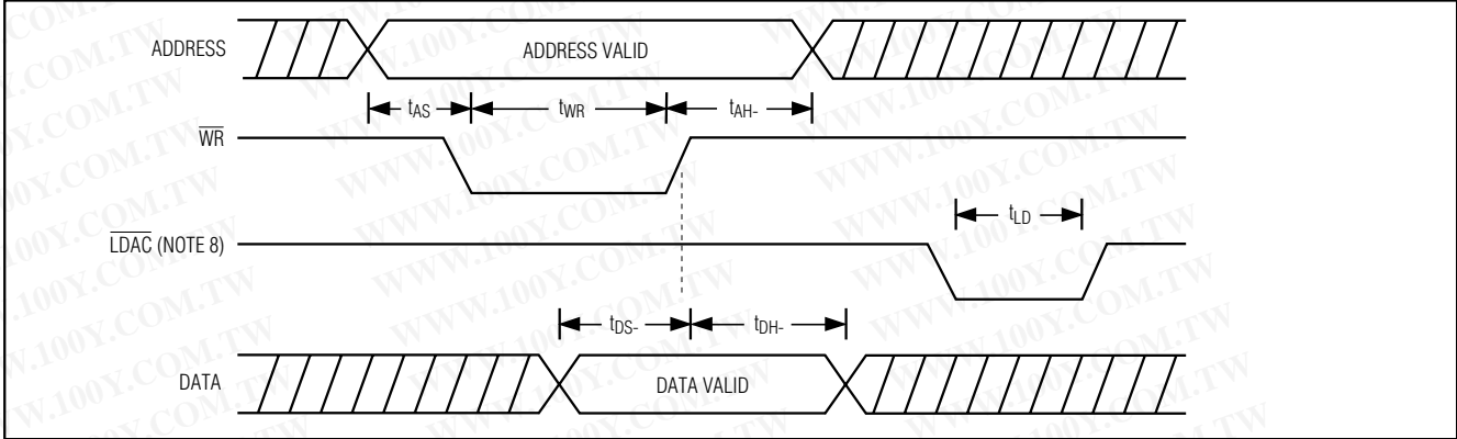
Figure 1. Timing Diagram
