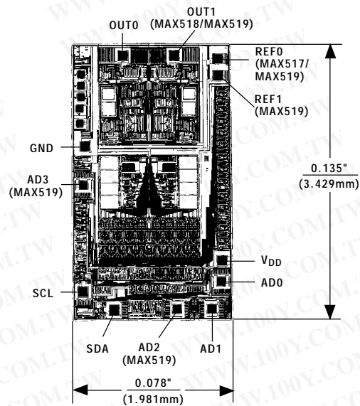
Chip Topography
