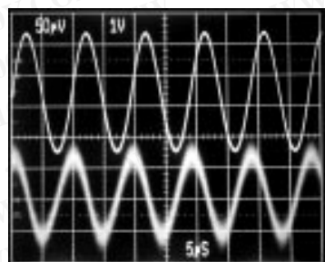
MAX517/MAX519 REFERENCE FEEDTHROUGH AT 100kHz
