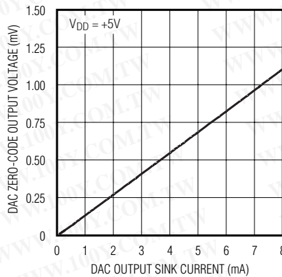
DAC ZERO-CODE OUTPUT VOLTAGE vs. OUTPUT SINK CURRENT
