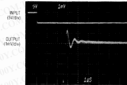
C_L = 100 pF, R_L = 5 k \Omega , V_{REF} = 2.5 V
