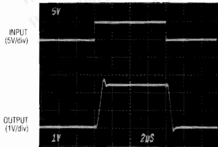
V_{DD} = +5 V, V_{SS} = -5 V, V_{REF} = 2.5 V, C_L = 100 pF, R_L = 5 k \Omega
