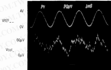
1ms/div TOP: REFERENCE IN 2V/div BOTTOM: V_{OUT} 20 \mu V/div INPUT CODE = ALL 0s
