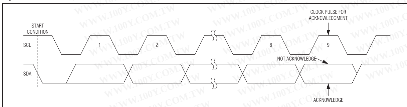
Figure 5. Acknowledge
