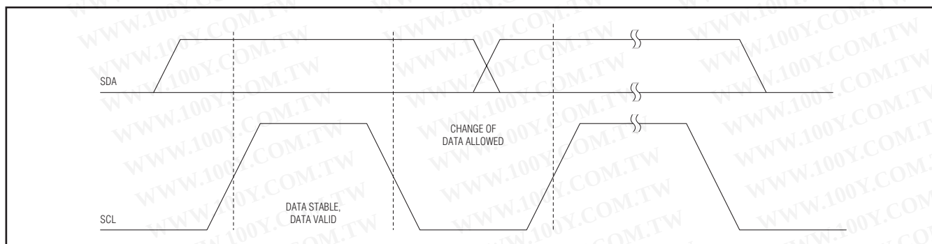
Figure 4. Bit Transfer
