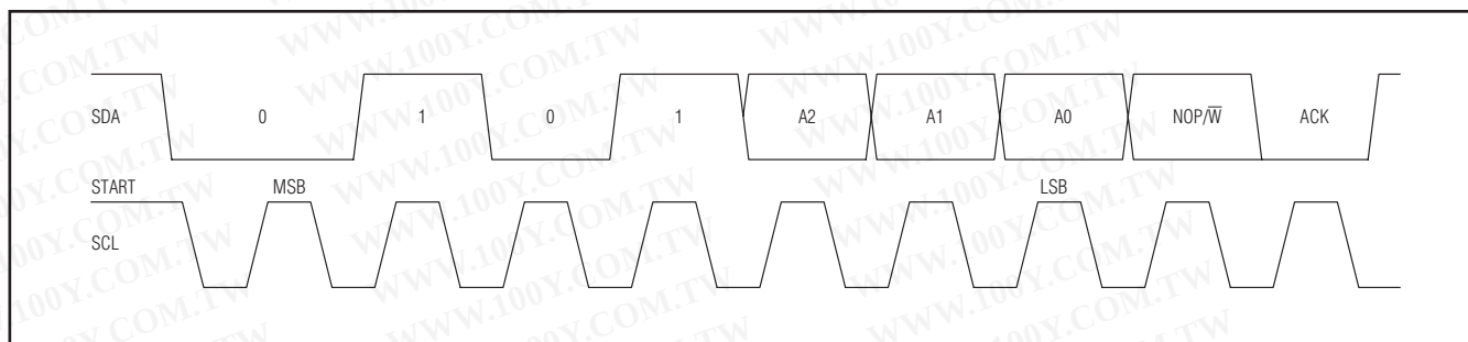
Figure 6. Slave Address
