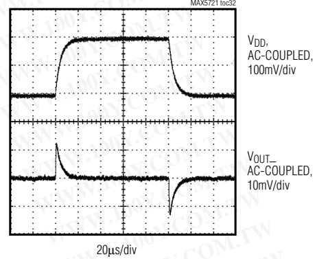
LINE TRANSIENT RESPONSE ( V_{DD} = +5\text{V} )
