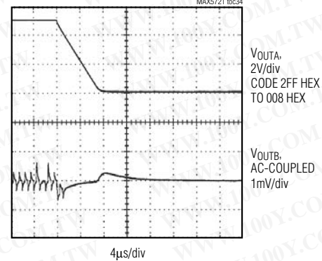
CROSSTALK ( V_{DD} = +5\text{V} )
