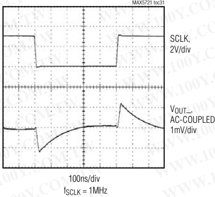
CLOCK FEEDTHROUGH ( V_{DD} = +3\text{V} )
