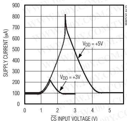
SUPPLY CURRENT vs. \overline{\text{CS}} INPUT VOLTAGE
