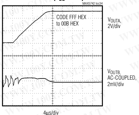
CROSSTALK ( V_{DD} = +5\text{V} )
