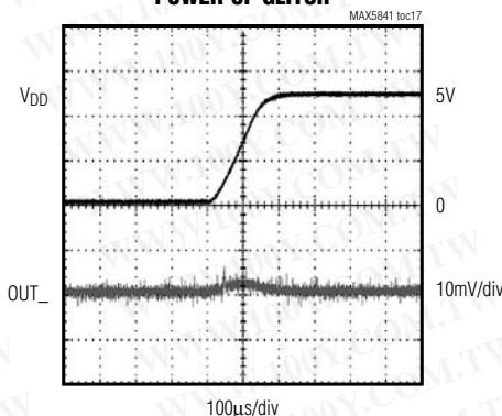
POWER-UP GLITCH
