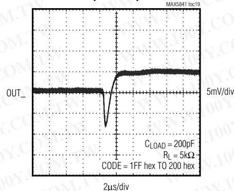
MAJOR CARRY TRANSITION (POSITIVE)
