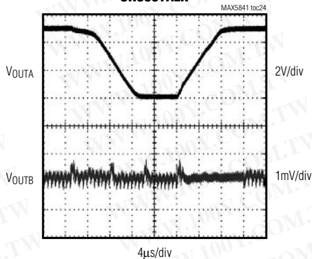
CROSSTALK
