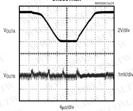
CROSSTALK
