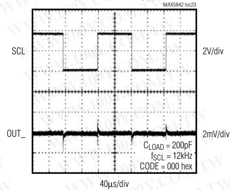
DIGITAL FEEDTHROUGH
