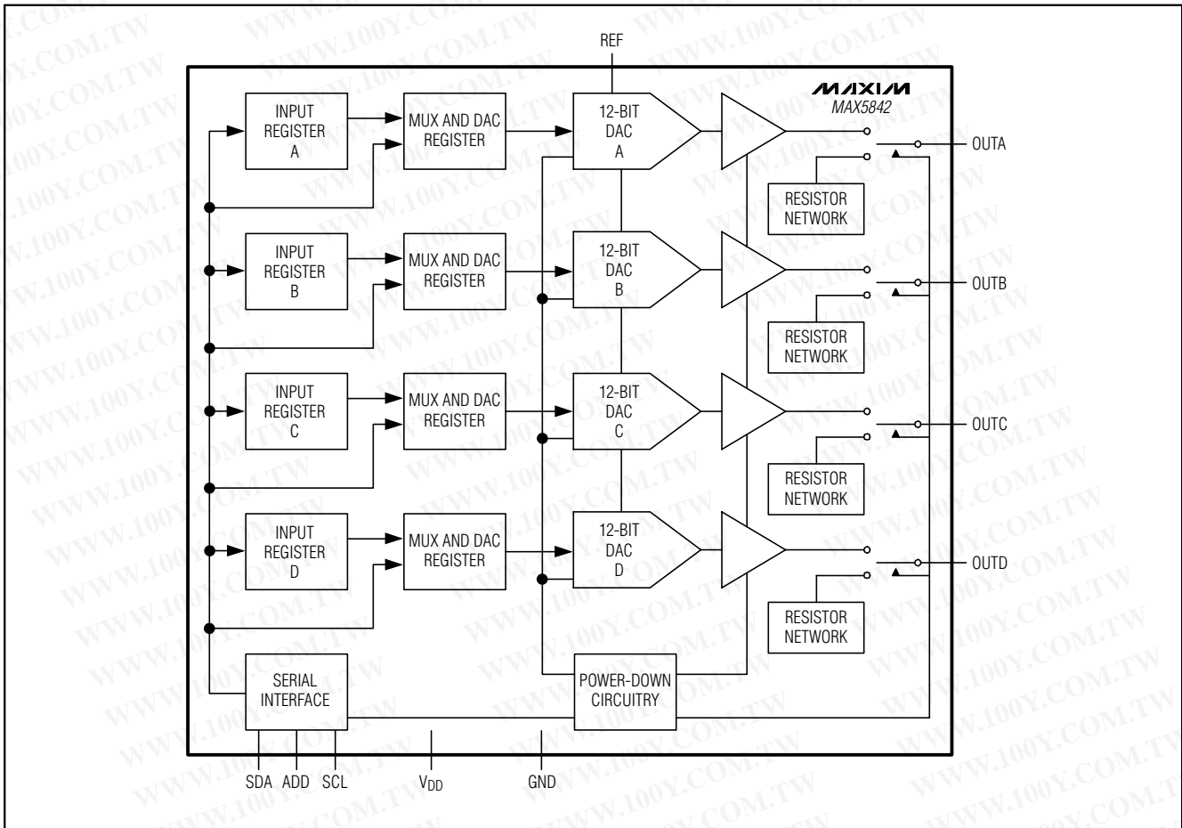
Functional Diagram
